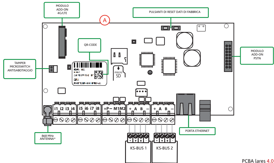
PCBA lares 4.0
